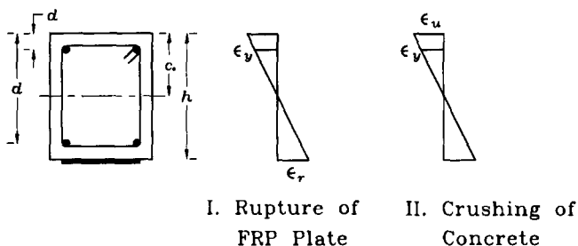
FIG. 5. Strain Diagram at Failure of Strengthened Beam
