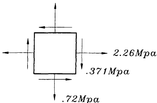
FIG. 10. Shear and Normal Stresses in Concrete at Cut-Off Point
