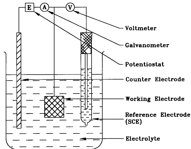
FIG. 4. Schematic of Electrical Circuitry for Polarization Measurement
