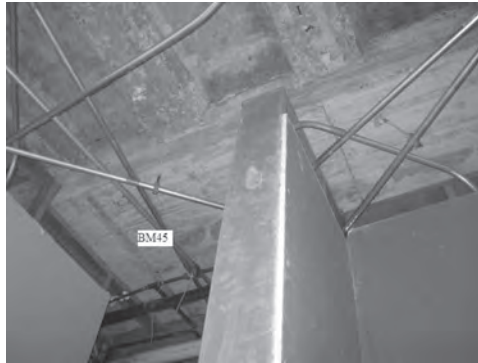
Figure 7 – Partition wall framing crossing the beam axis
