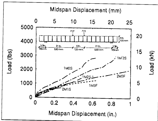
Fig. 7—Load versus deflection for retrofitted URM beams
